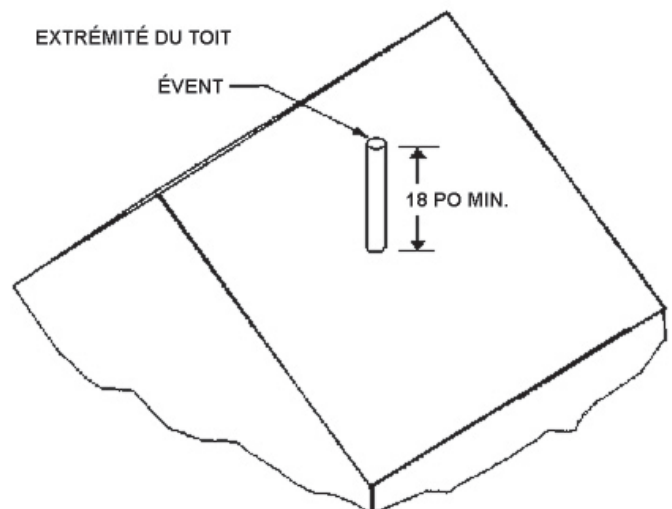
Figure 10 - Ventilation verticale
