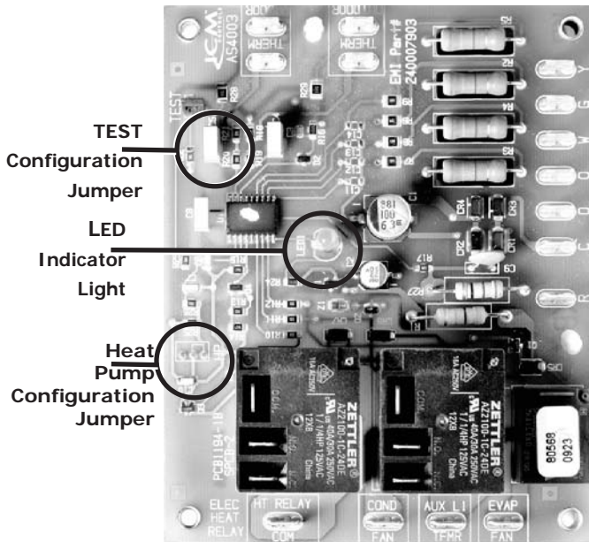
Figure 8 Control Board
