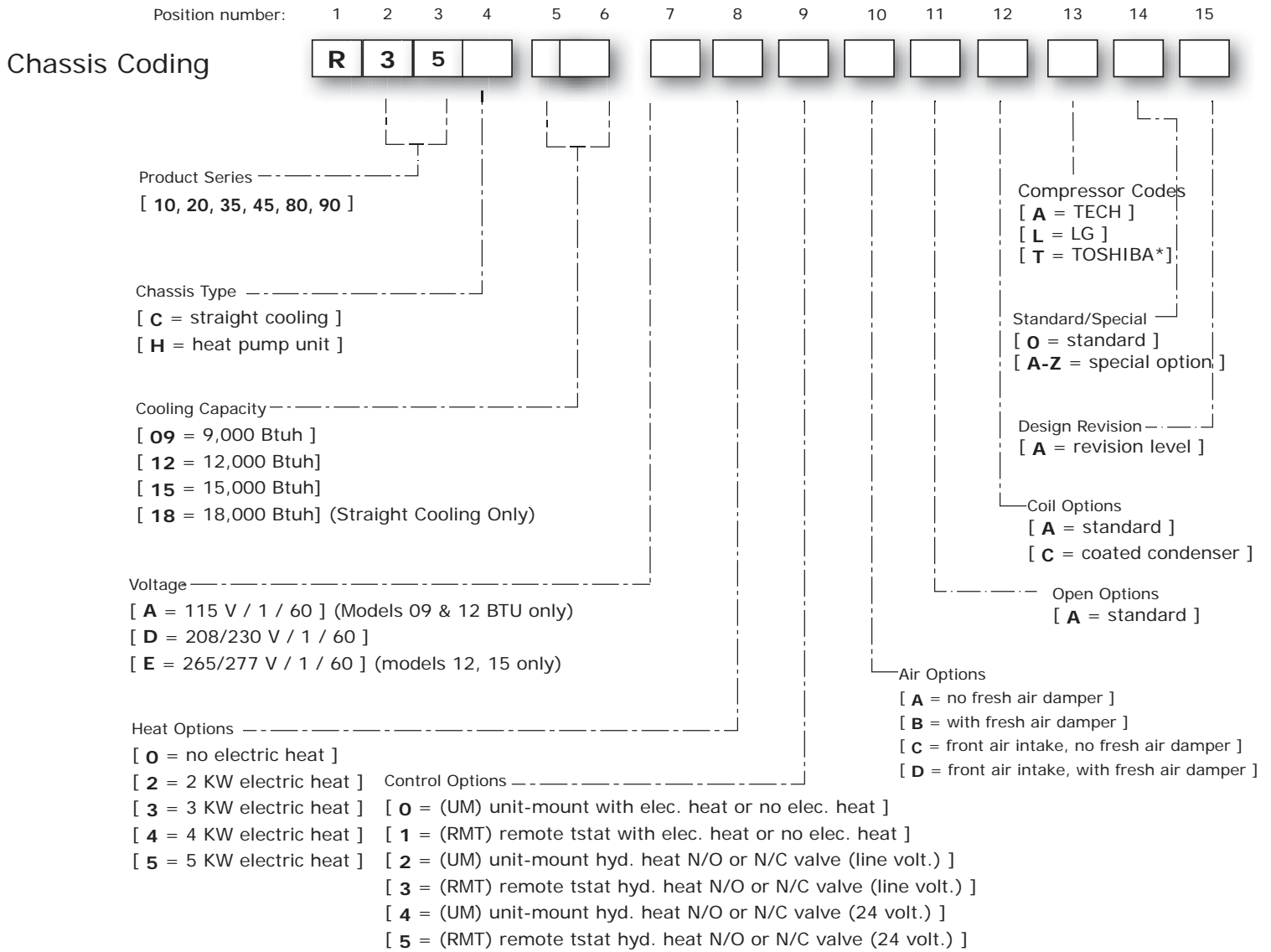
Figure 5 Model Coding
