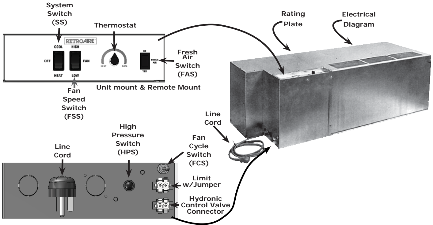
Figure 2 R80C | R80H Chassis
