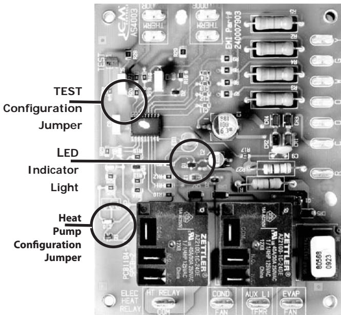
Figure 4 Control Board
