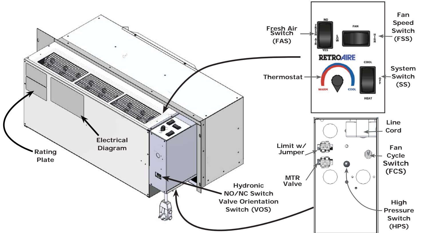
Figure 2 R11C Chassis
