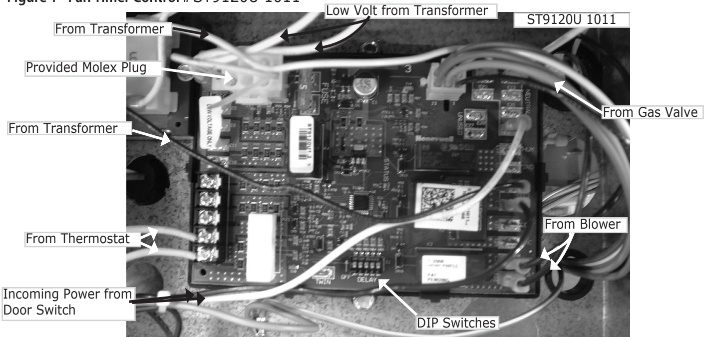
Figure 1 - Fan Timer Control # ST9120U 1011
