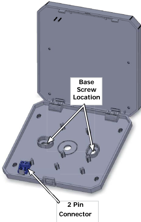
Figure - 4 User Interface 2 Pin Connector
