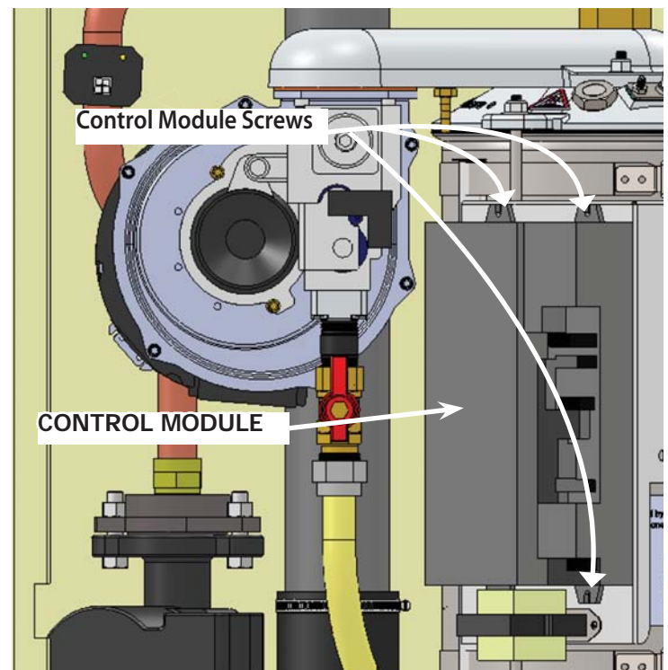
Figure 2 - Control Module
