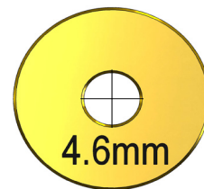
Figure - 3 Orifice de gaz de PL type
