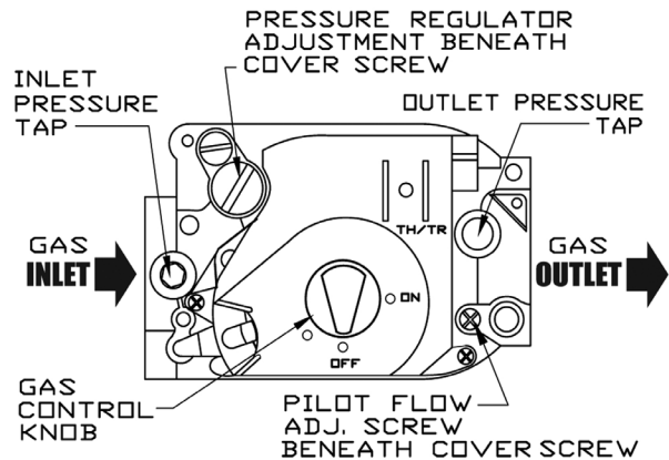
Figure 3 - Gas Valve
