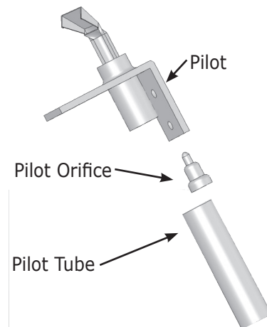
Figure 2 - Pilot Assembly
