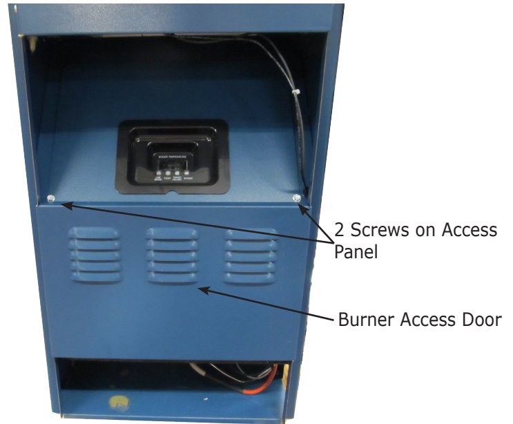
Figure 1 Burner Door and Control Access Panel
