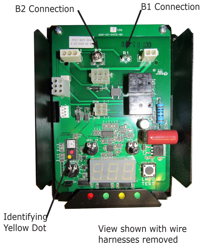
Figure 2 Control
