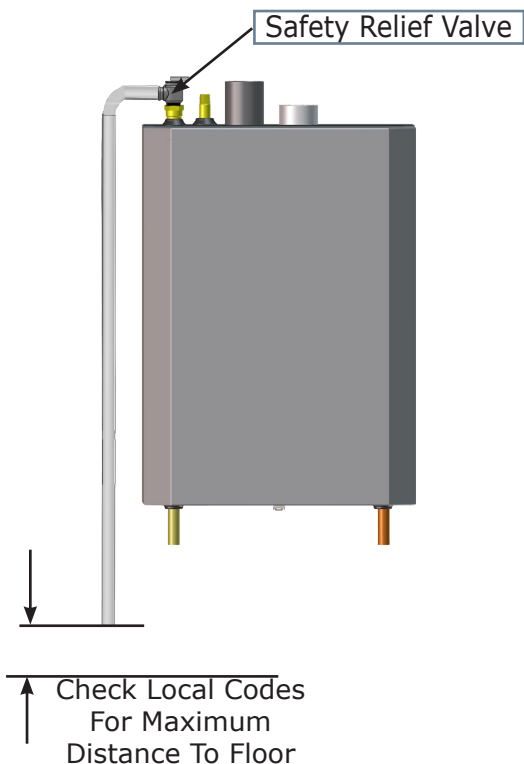
FIGURE 6-2 Safety Relief Valve Discharge Piping
