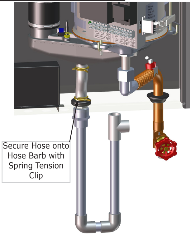
FIGURE 6-1 Condensate Drain
