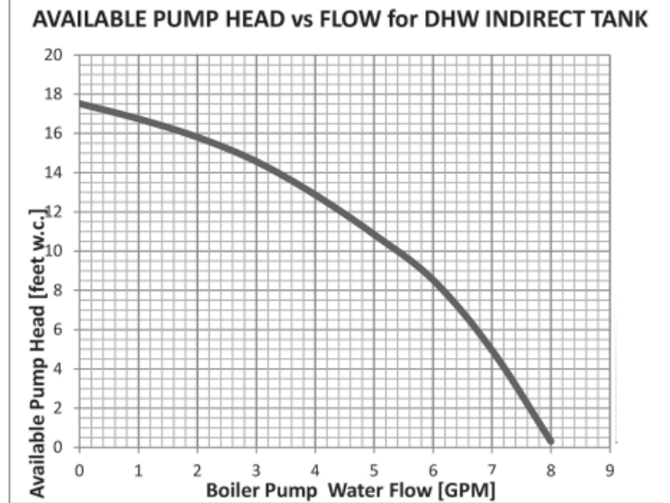
Figure 7 - Indirect Tank Performance Chart
