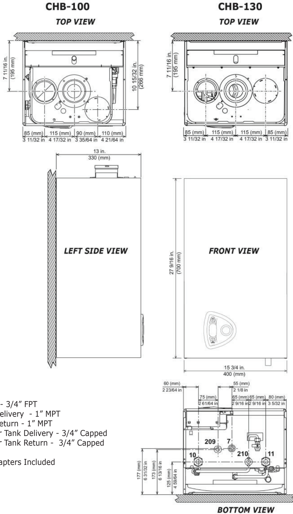
Figure 1 - Overall Dimensions
