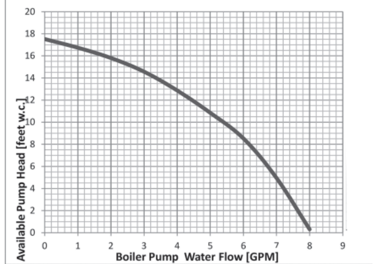
Figure 7 - Diagramme de performance du ballon indirect AVAILABLE PUMP HEAD for DHW INDIRECT TANK
