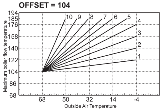
- Compensation curves
