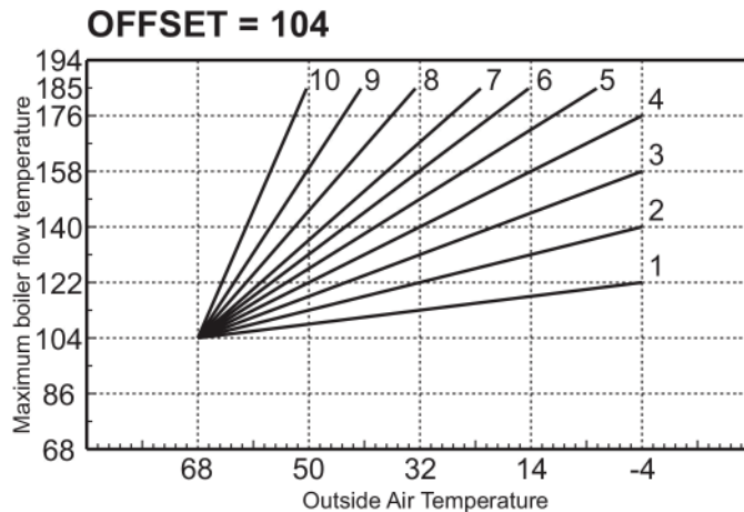
- Compensation curves
