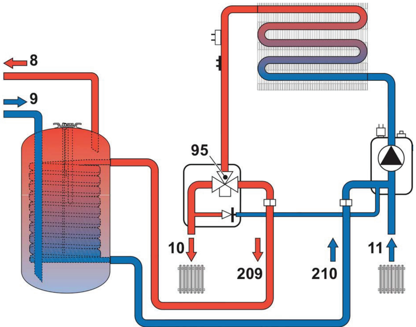
Figure 10 - Tuyauterie hydronique
