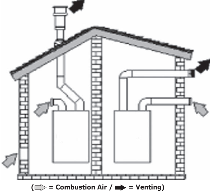
Figure 13 - Two Pipe Venting
