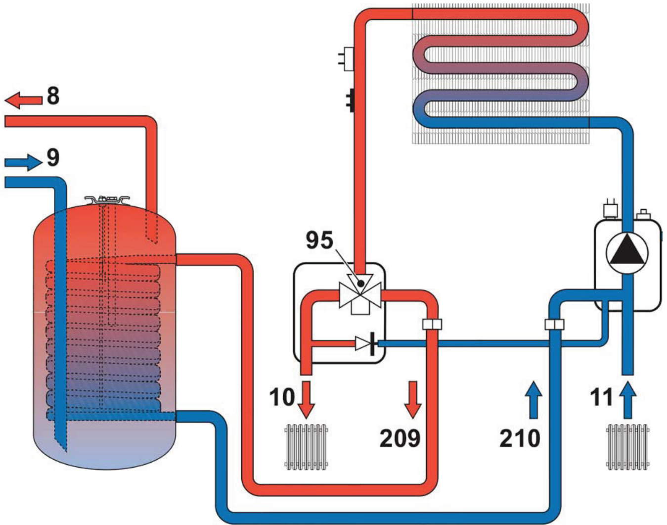
Figure 10 - Hydronic Piping
