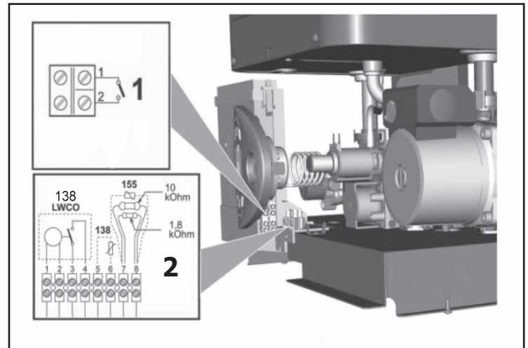
Figure 17 - Terminal Block
