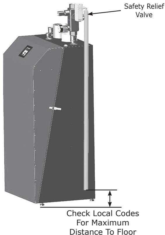
FIGURE 6-2 Safety Relief Valve Discharge Piping
