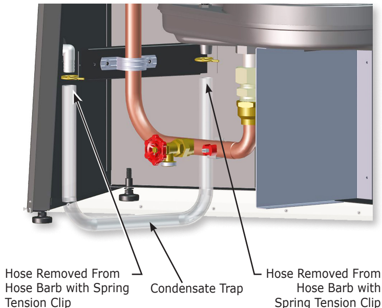
FIGURE 6-1 Condensate Drain - Option Left or Right Side
