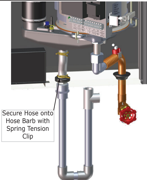
FIGURE 5-1 Condensate Drain
