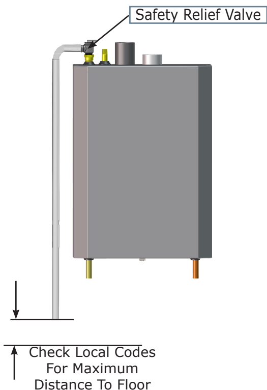
FIGURE 5-2 Safety Relief Valve Discharge Piping
