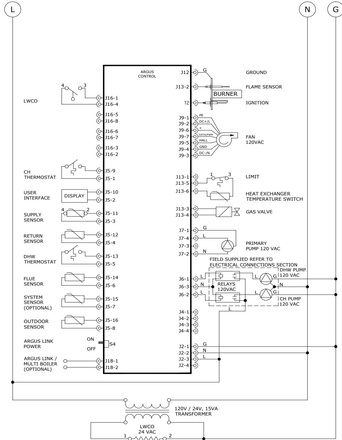
LADDER DIAGRAM 50/75/100
