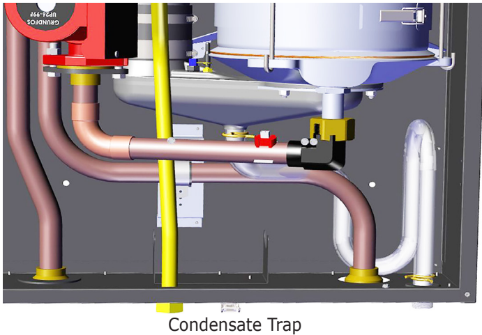
FIGURE 5-1 Condensate Drain
