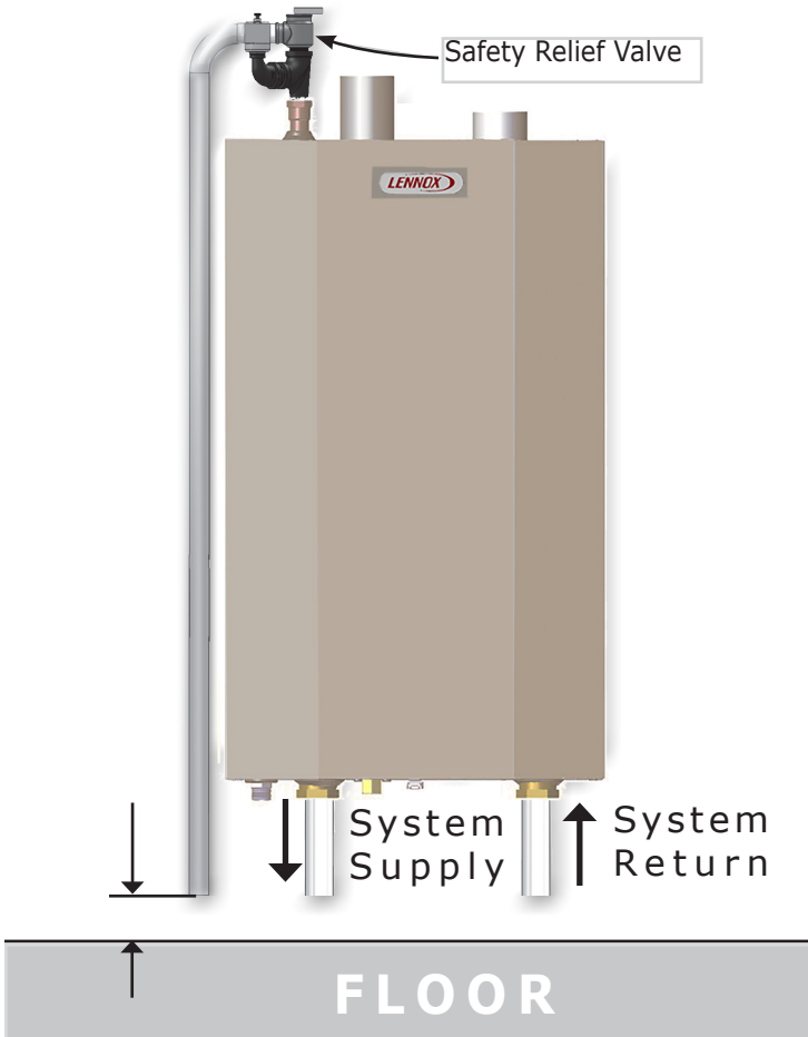
FIGURE 5-2 Safety Relief Valve Discharge Piping
