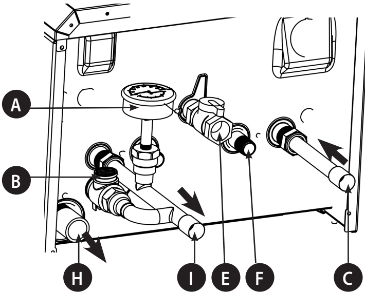
HEATING ONLY WITHOUT OPTIONAL INDIRECT DHW CONNECTION
