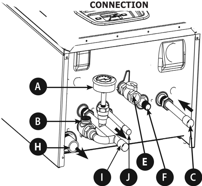
HEATING ONLY WITHOUT OPTIONAL INDIRECT DHW CONNECTION
