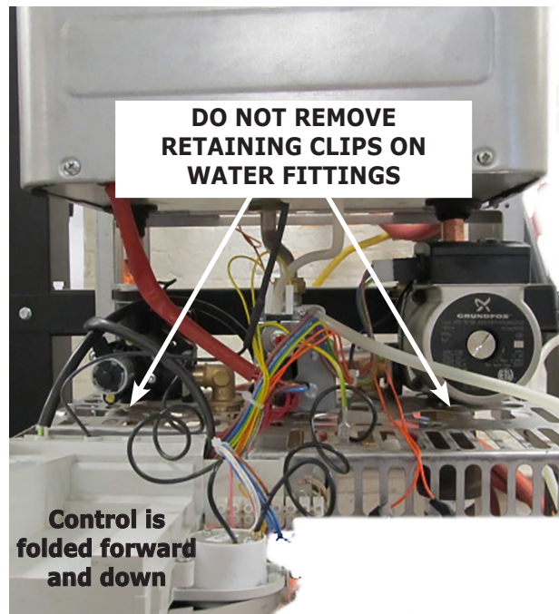
Boiler shown with jacket removed
