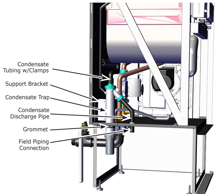
Figure 2 - Condensate Trap - (Left and front panels removed for illustration only)
