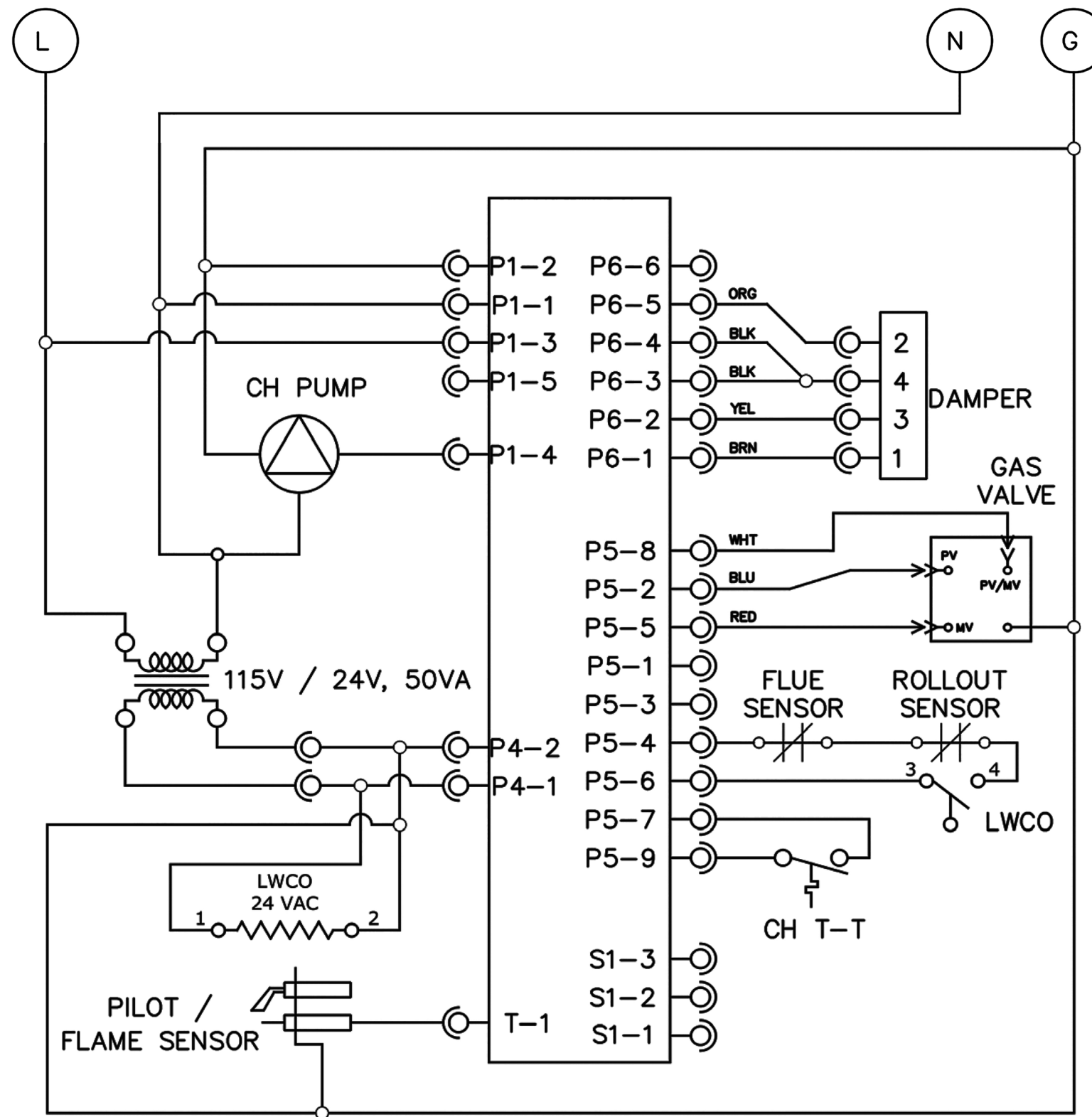
LADDER DIAGRAM: HOT WATER - ATMOSPHERIC DRAFT BOILER
