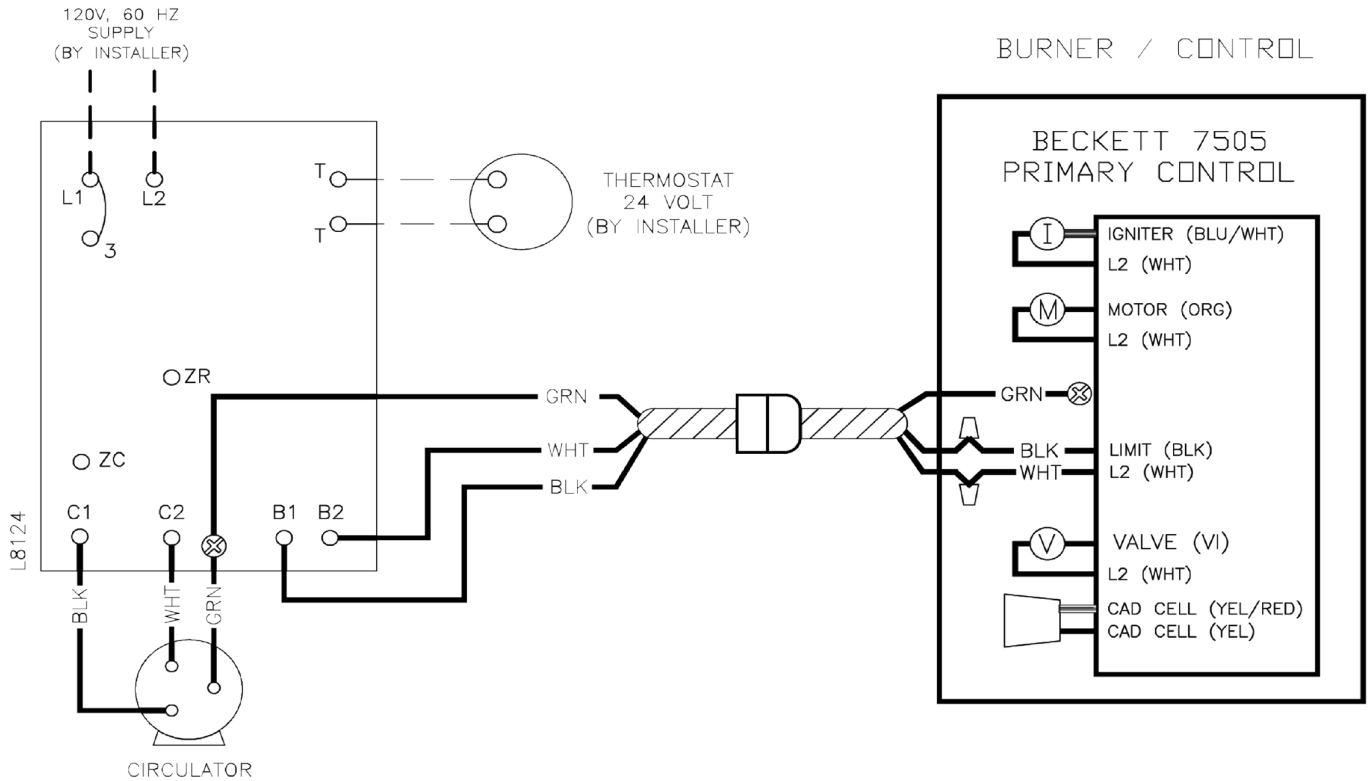
Figure 2 -Wiring Diagram Beckett AFG with Tankless Heater
