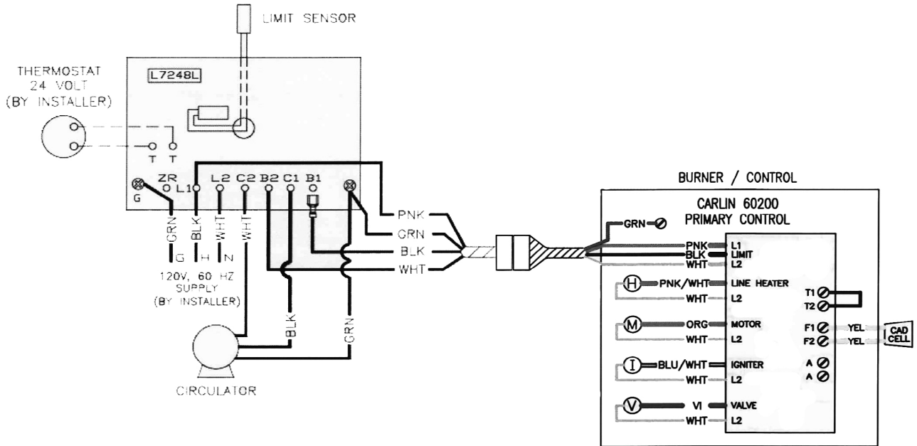
Figure 7 - Wiring Diagram Carlin EZ-1/2 without Tankless Heater
