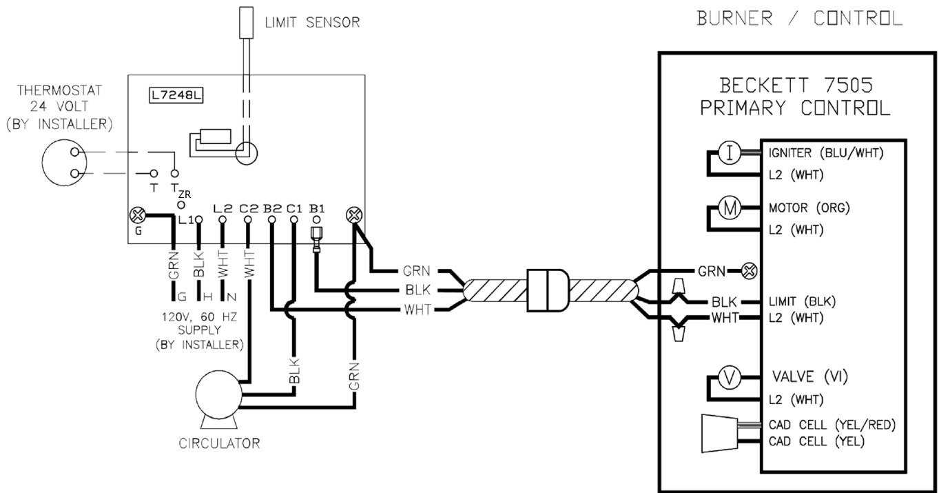
Figure 2 -Wiring Diagram Beckett AFG with Tankless Heater
