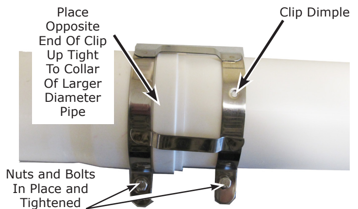
Figure 3 - Vent Clip Orientation
