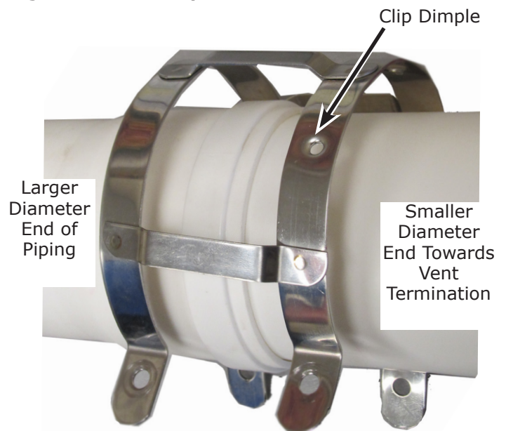
Figure 3 - Vent Clip Orientation
