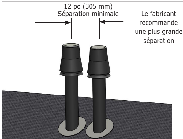
FIGURE 6-3 – Évacuation coaxiale verticale
