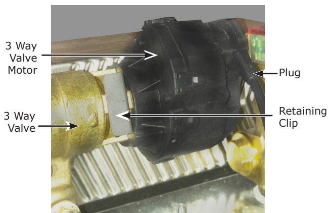
Figure 3 - Combi 3 Way Valve Motor
